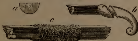
a , Section of bow; b , end of bow, showing nock; c , handle of bow.
